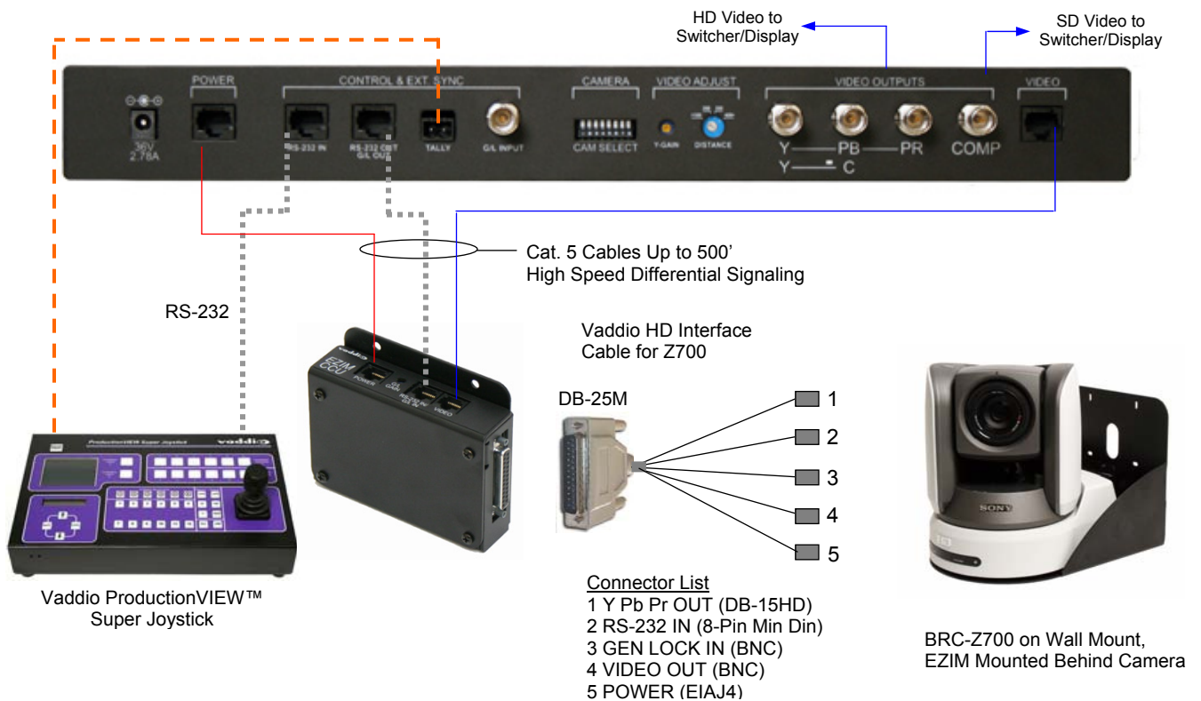
Figure 4: Basic system connectivity of a WallVIEW CCU Z700 System and ProductionVIEW Super Joystick Controller
