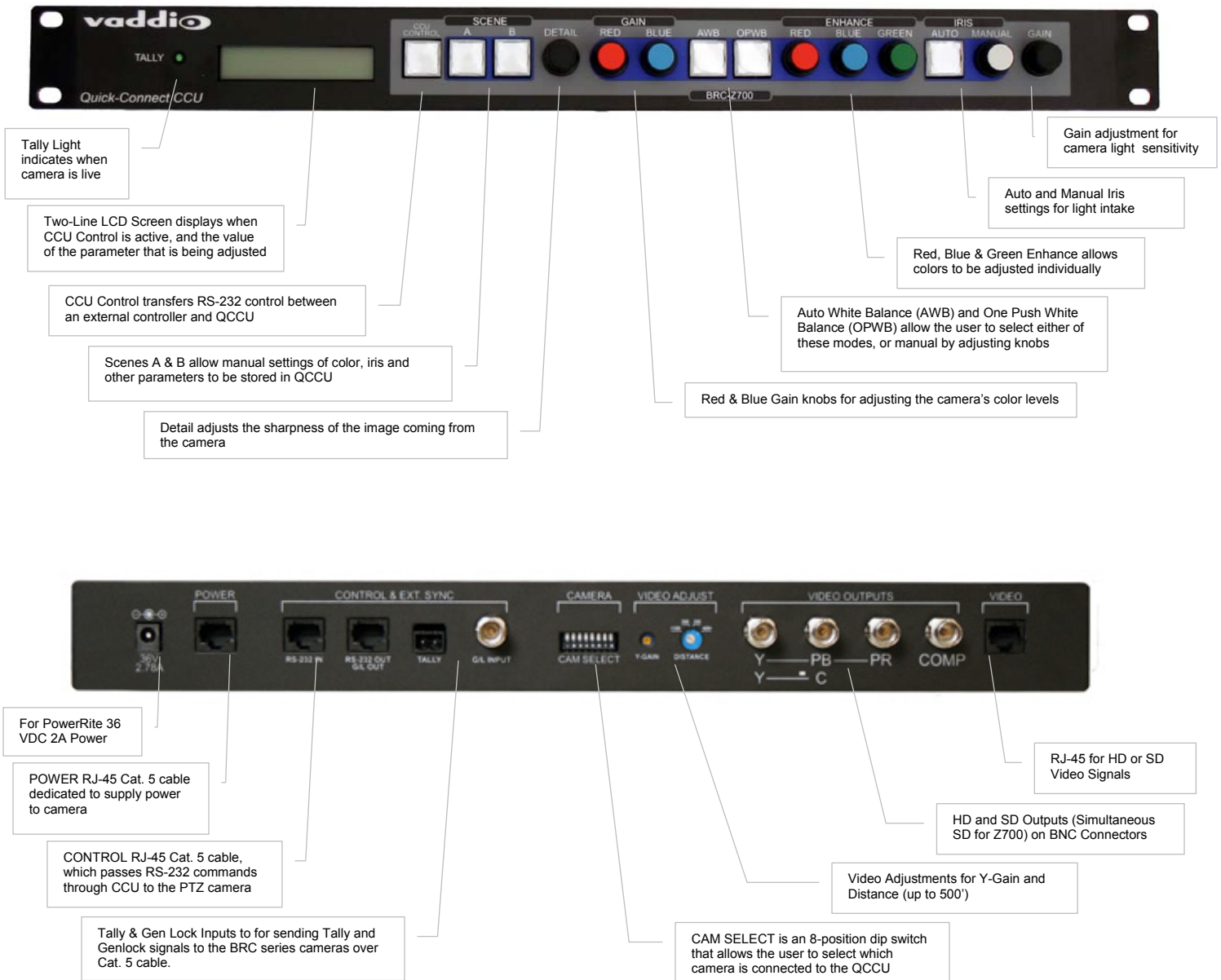
Figure 2: Quick-Connect CCU (QCCU) interface front panel and rear panel diagrams with functional callouts.
