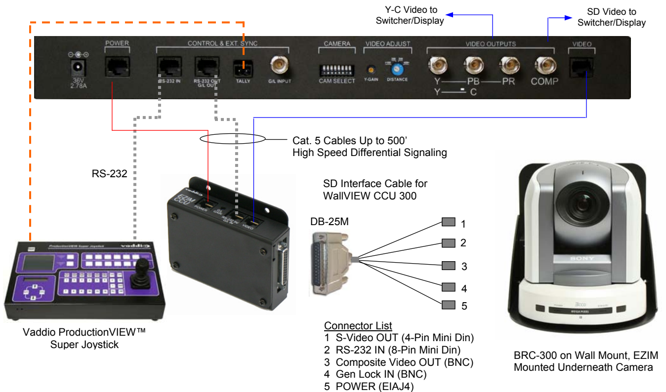
Figure 4: Basic system connectivity of a WallVIEW CCU 300 System and ProductionVIEW Super Joystick Controller
