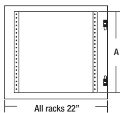
Front View shown without door
