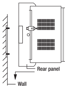
Side View Mounting Detail
