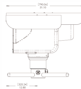
EOSS 825-S Side View
